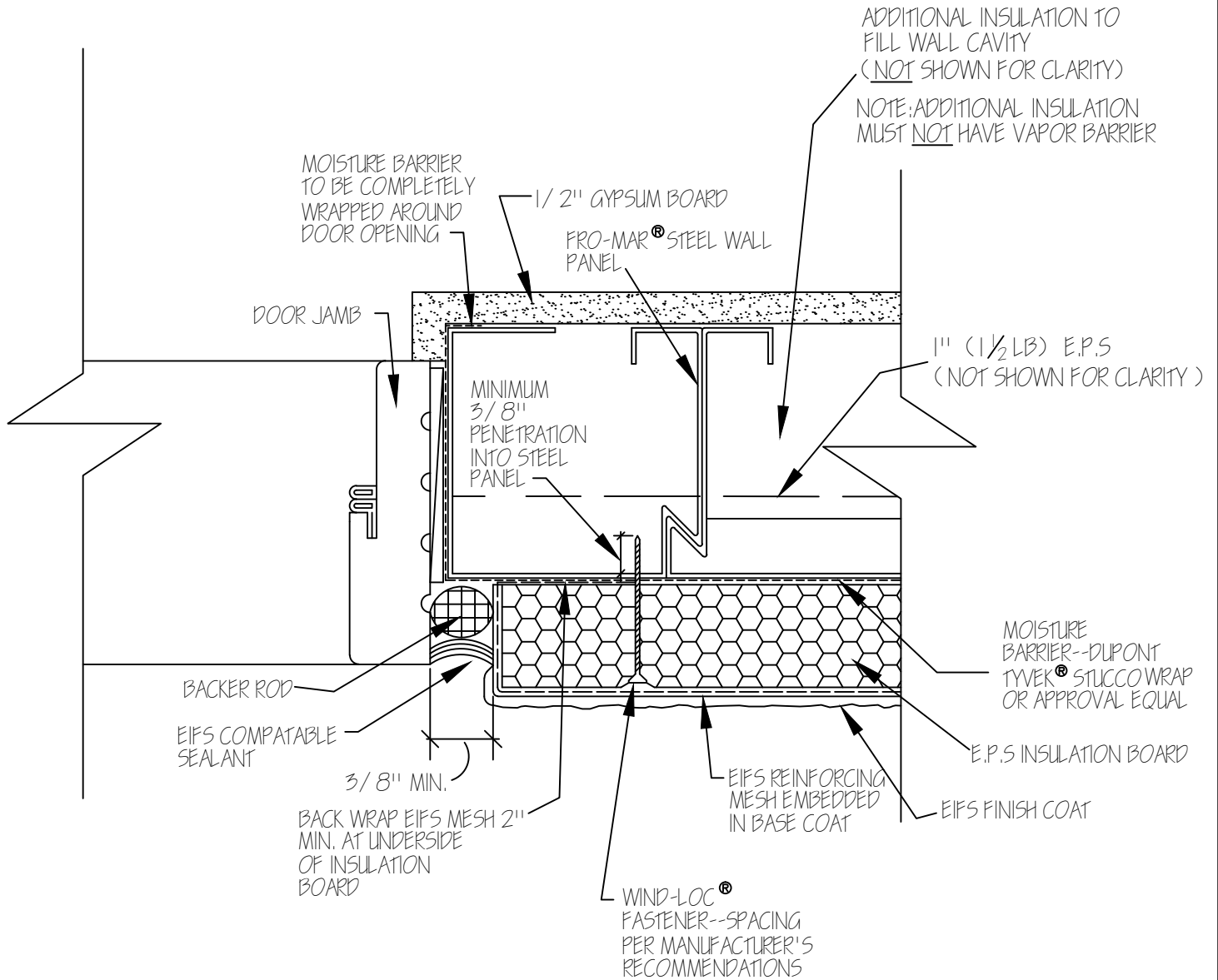
SUGGESTED DOOR JAMB DETAIL FOR EIFS
